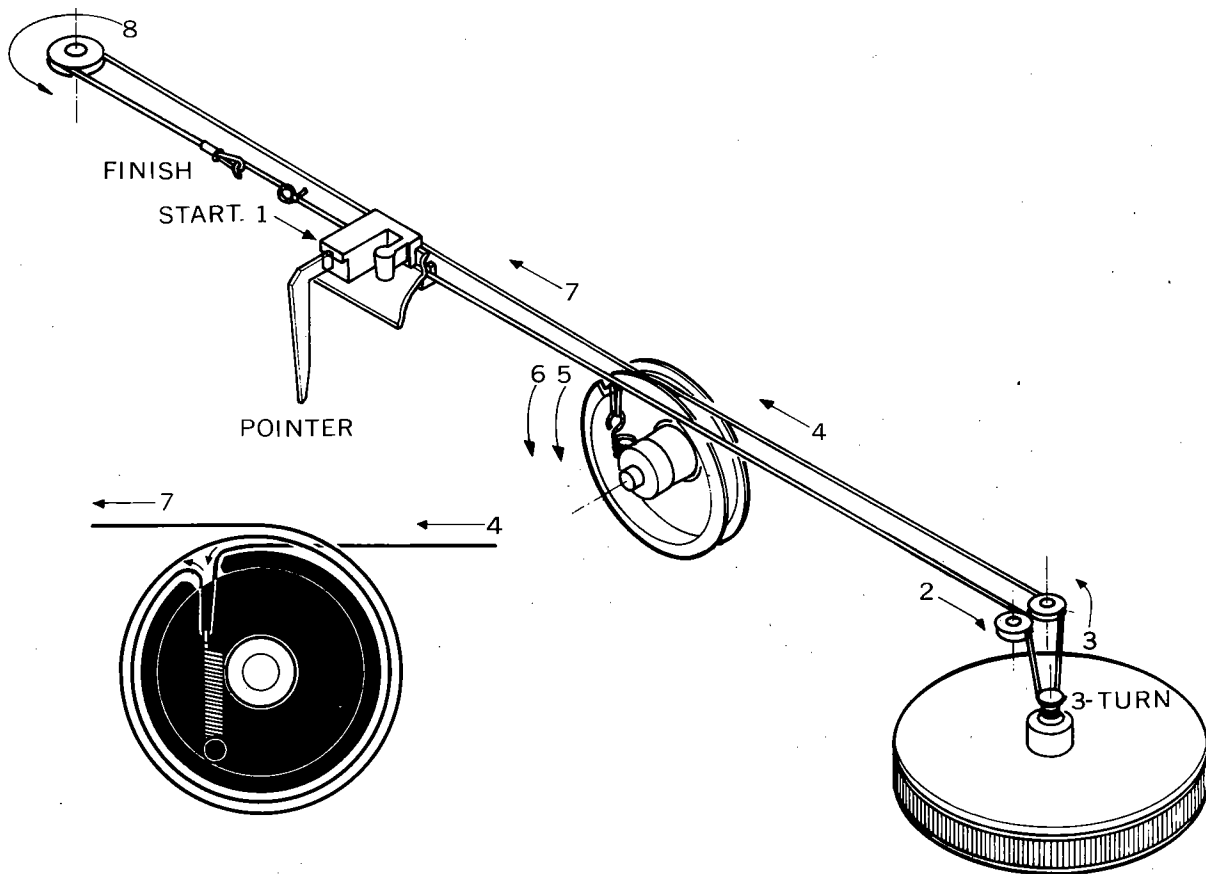
Figure 4 Dial Stringing
