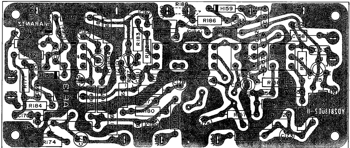
Figure 14 AM Tuner Unit Assembly P150 Component Locations
