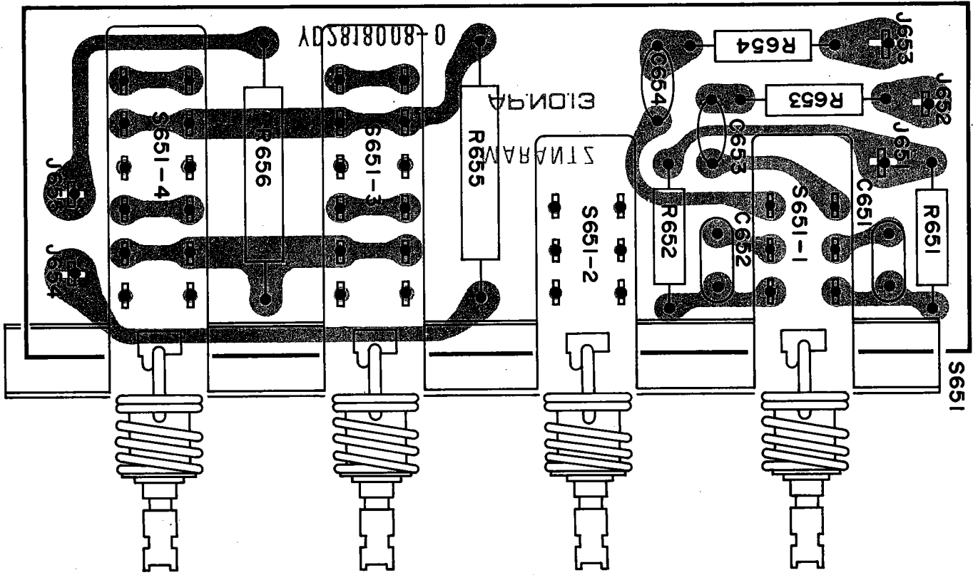
Figure 21 Loudness, Muting and Speakers Switch Assembly P650 Component Locations
