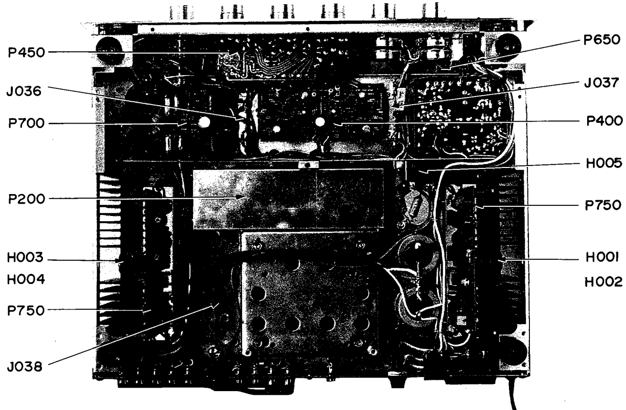
Figure 8 Main Chassis Component Locations (Bottom View)
