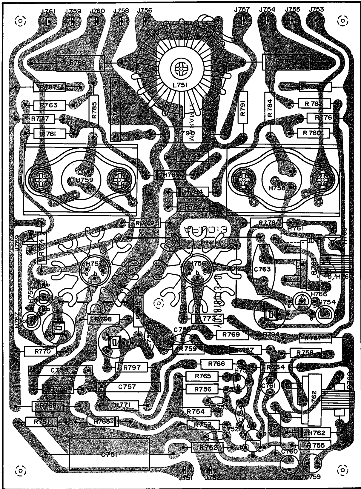
Figure 18 Power Amplifier Assembly P750 Component Locations
