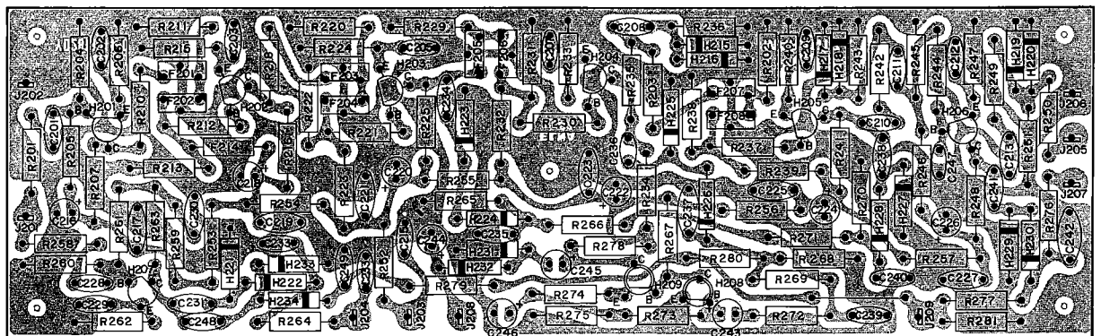
Figure 10 FM IF Amplifier Assembly P200 Component Locations
